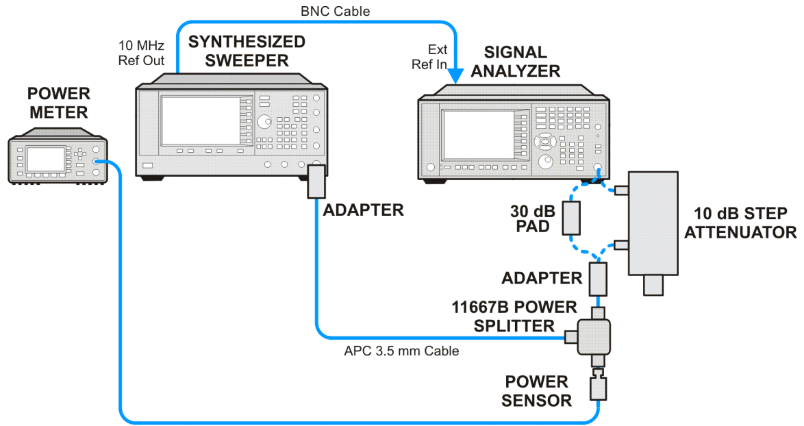
Figure 4-1. Amplitude Accuracy Test Setup
